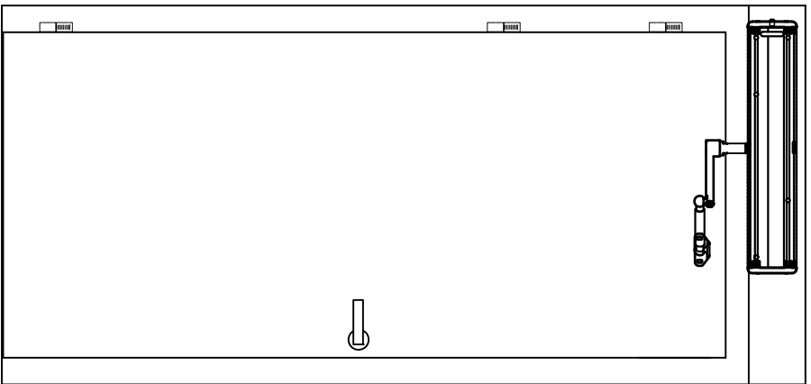
ADSF SPRINT SWING DOOR OPERATOR - LIGHT DUTY INTERNAL USE PUSH ARM (OPEN OUTWARDS) CONFIGURATION FRONT ELEVATION
